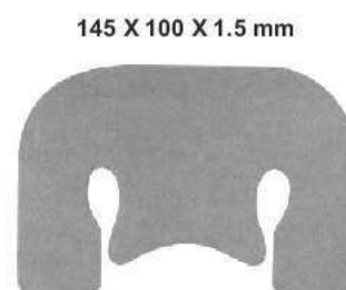
14-157 Silicon operating pad pre-cut
